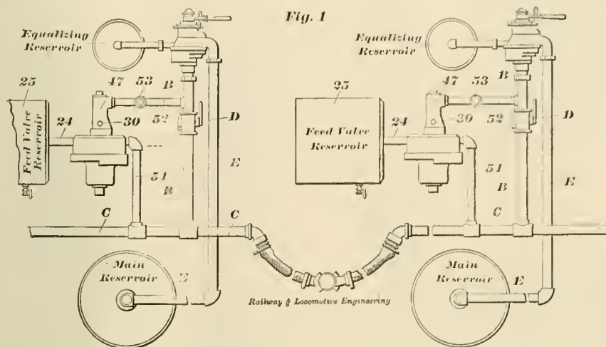
RECENTLY INVENTED AUTOMATIC DOUBLE HEADING FEED VALVE.
